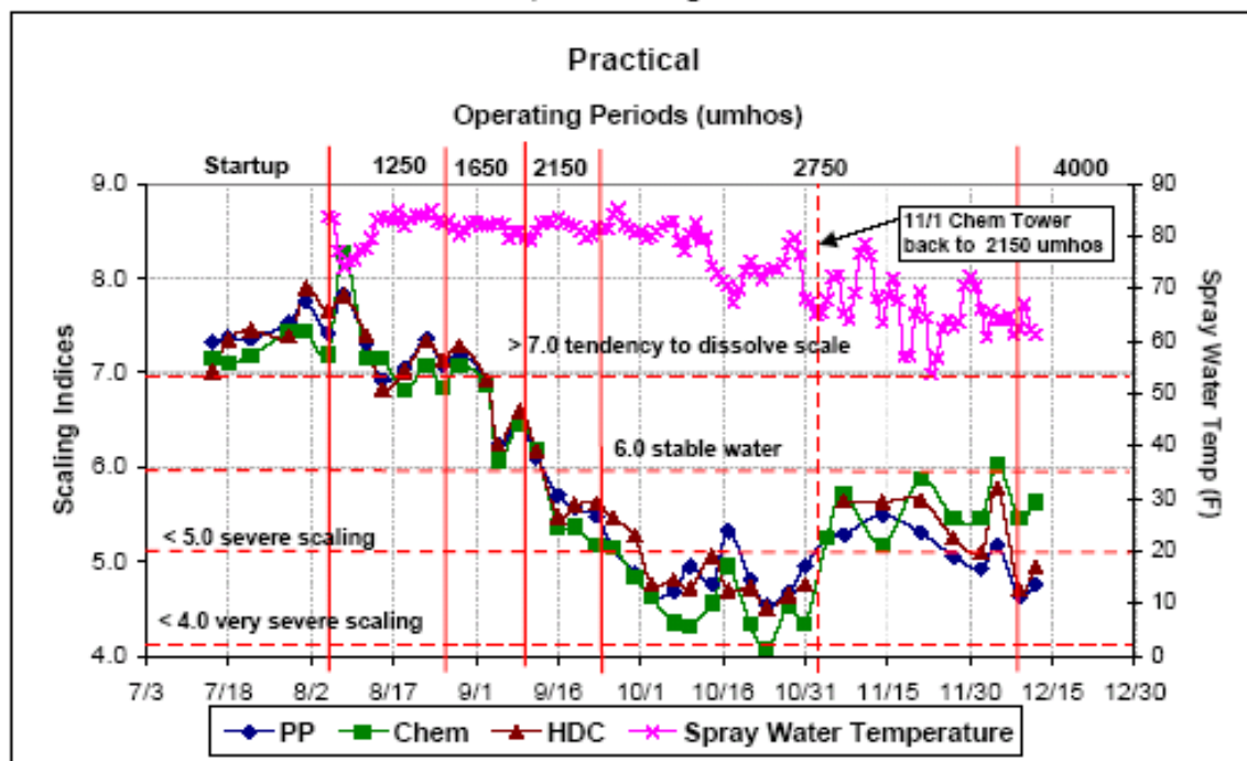
Figure 8. Practical Scaling Index
