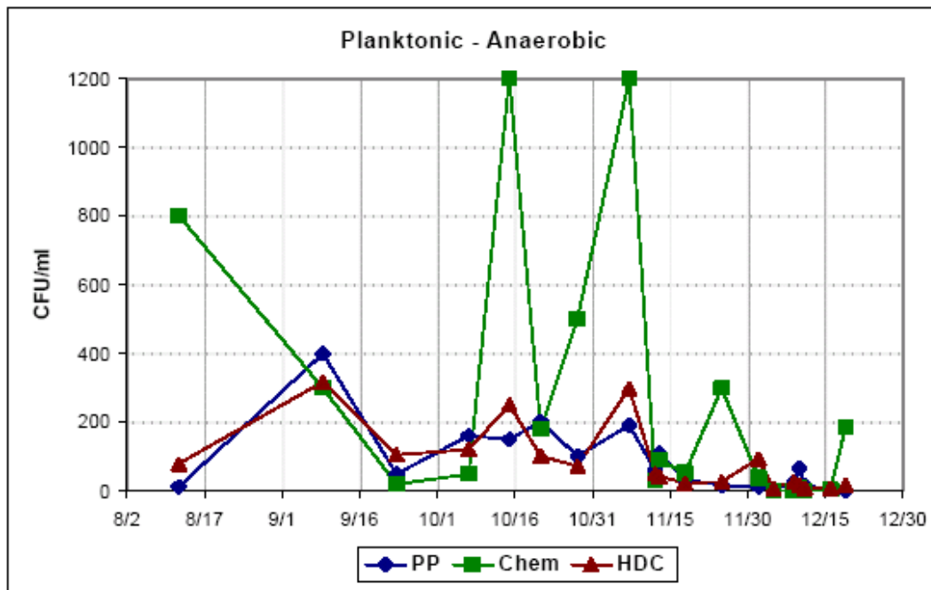
Figure 16. Planktonic Counts – Anaerobic History
