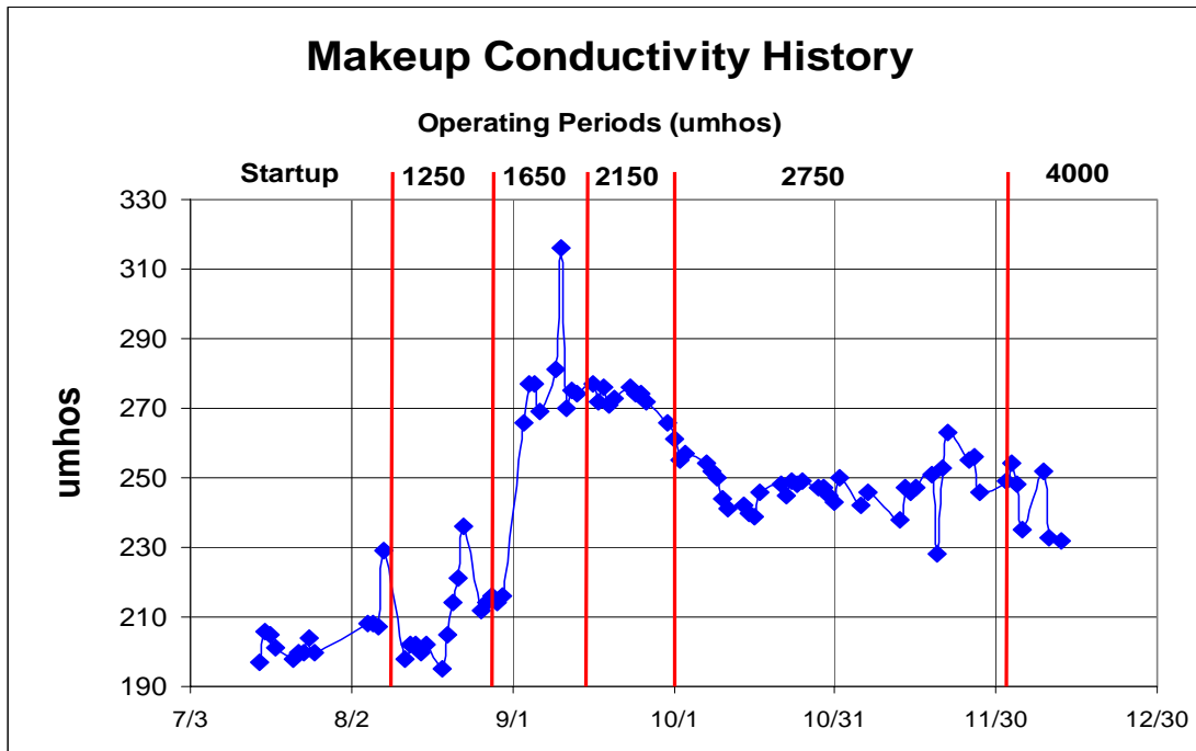
Figure 4. History of Makeup Conductivity
