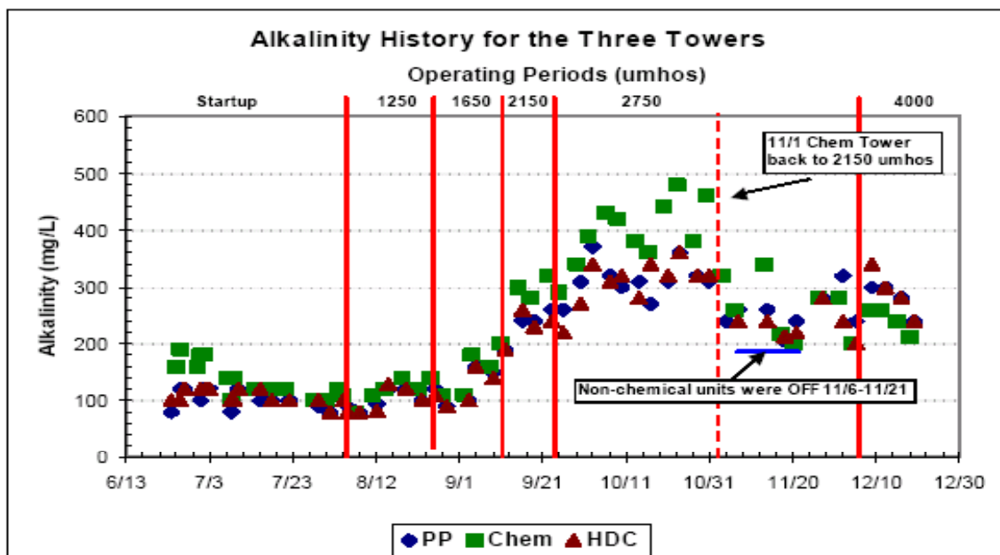
Figure 9. Alkalinity History
