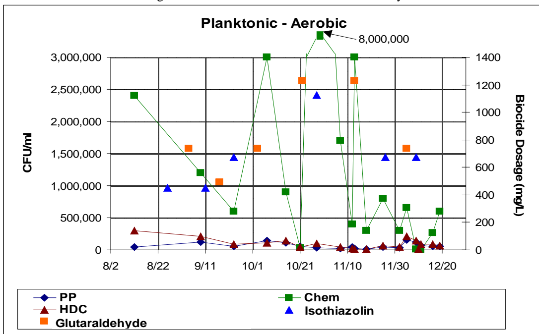
Figure 15. Planktonic Counts – Aerobic History
