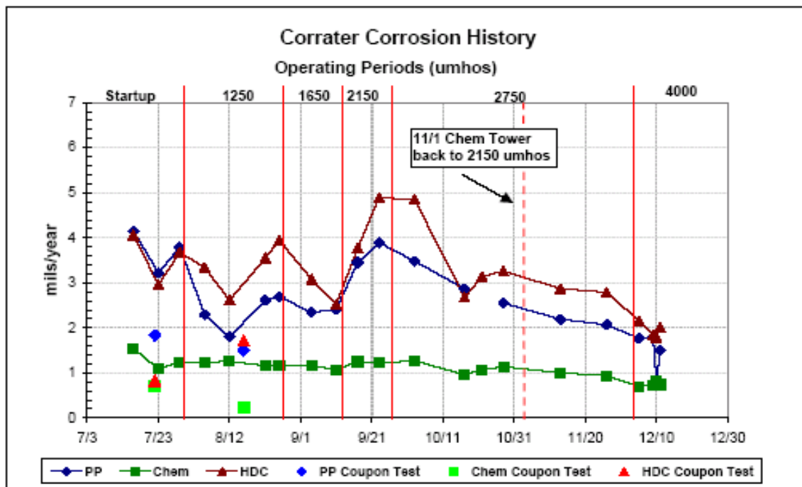
Figure 7. Corrat ® Corrosion History
