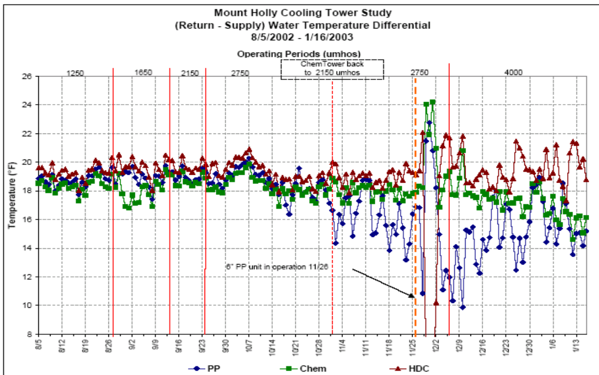
Figure 11. Return - Supply Water Temperature Differential
